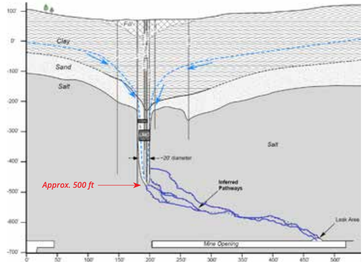
Before Grout: Water was leaking into the mine at approximately 45m 3 /hr
